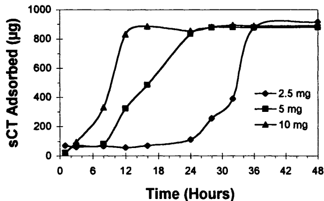
Fig. 1. Time course of sCT adsorption to PLGA at various microsphere concentrations. Microspheres were suspended in a 1 \text{ mg}/\text{ml} sCT solution in 0.01 \text{ M} phosphate buffer, \text{pH } 7.4 .
