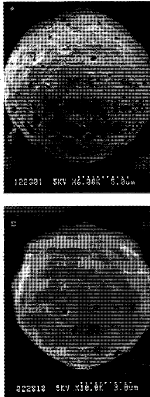
Fig. 2. Scanning electron micrographs of blank PLGA microspheres (A): Before adsorption, (B): Suspended in phosphate buffer, \text{pH } 7.4 , containing sCT for 6 days.
